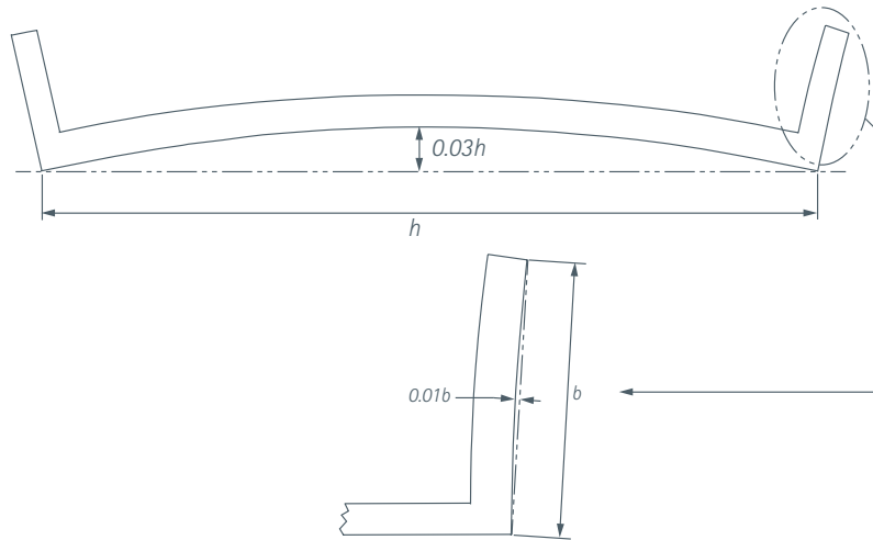
Figure 52 – Measurement of flatness
