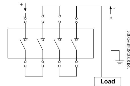
H) 4 poles in series (1000 Vdc)
