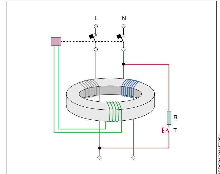
Figure 1: Operating principle of the residual current device
