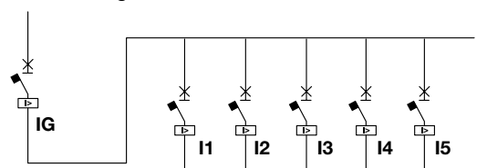
Circuit diagram
