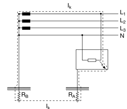
Figure 1: Earth fault in TT system
