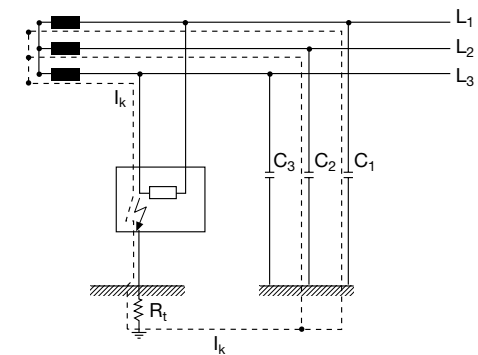
Figure1: Earth fault in IT system
