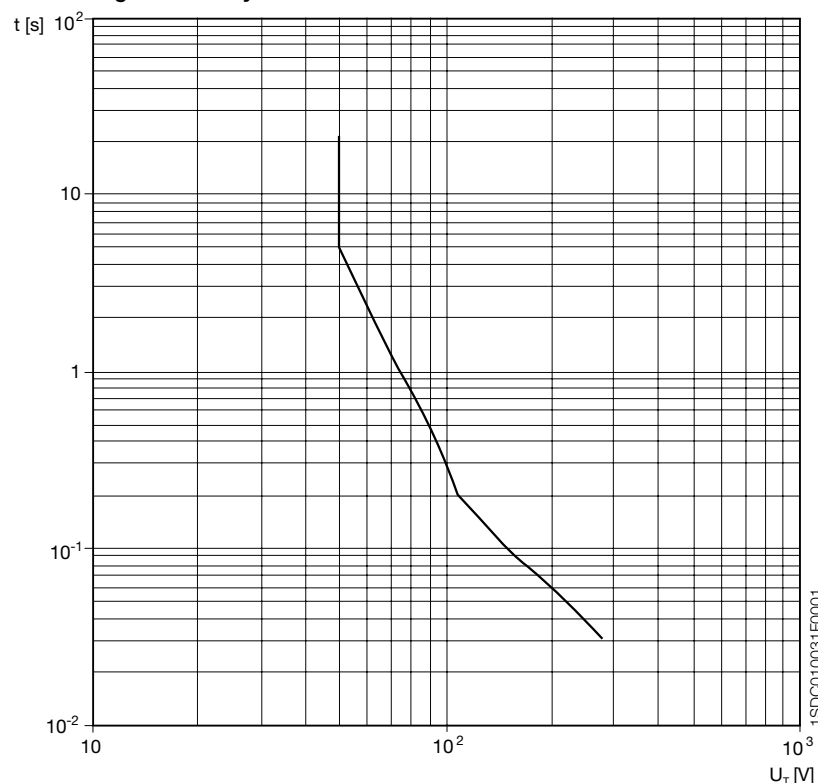
Figure 2: Safety curve
