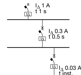
Figure 3: Vertical discrimination between RCDs
